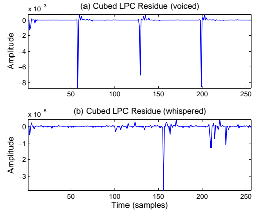
Figure 4: Cubed LPC Residues for (a) voiced and (b) whispered segments. After cubing the residue, the voiced residual exhibited a distinct periodic structure useful for estimating the amount of periodicity in the waveform.
