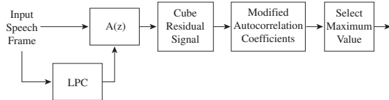
Figure 3: Algorithm for extracting the MLPCs.
